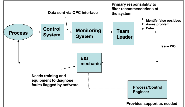
Figure 10 – shows a realistic view of the workflow using a Loop Monitoring system
