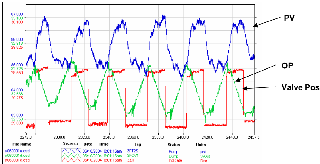
Figure 2 – Process variability caused by stiction
