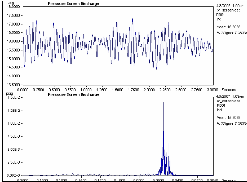
Figure 1 High frequency process variability
