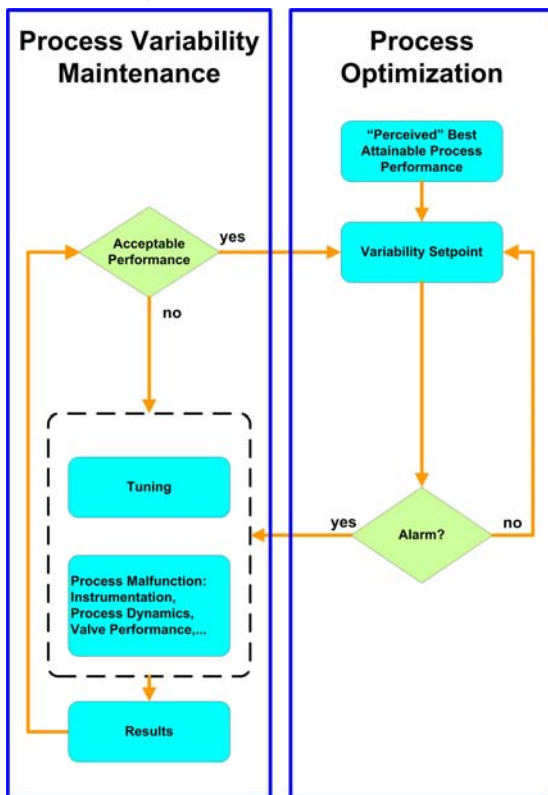
Figure 6 the loop monitoring system plays a central role in the idealized view.
