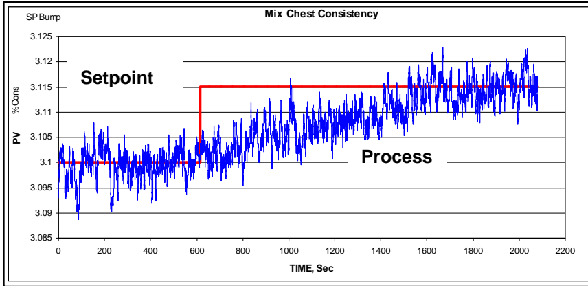
Figure 3 – Unnecessarily slow tuning on a consistency loop
