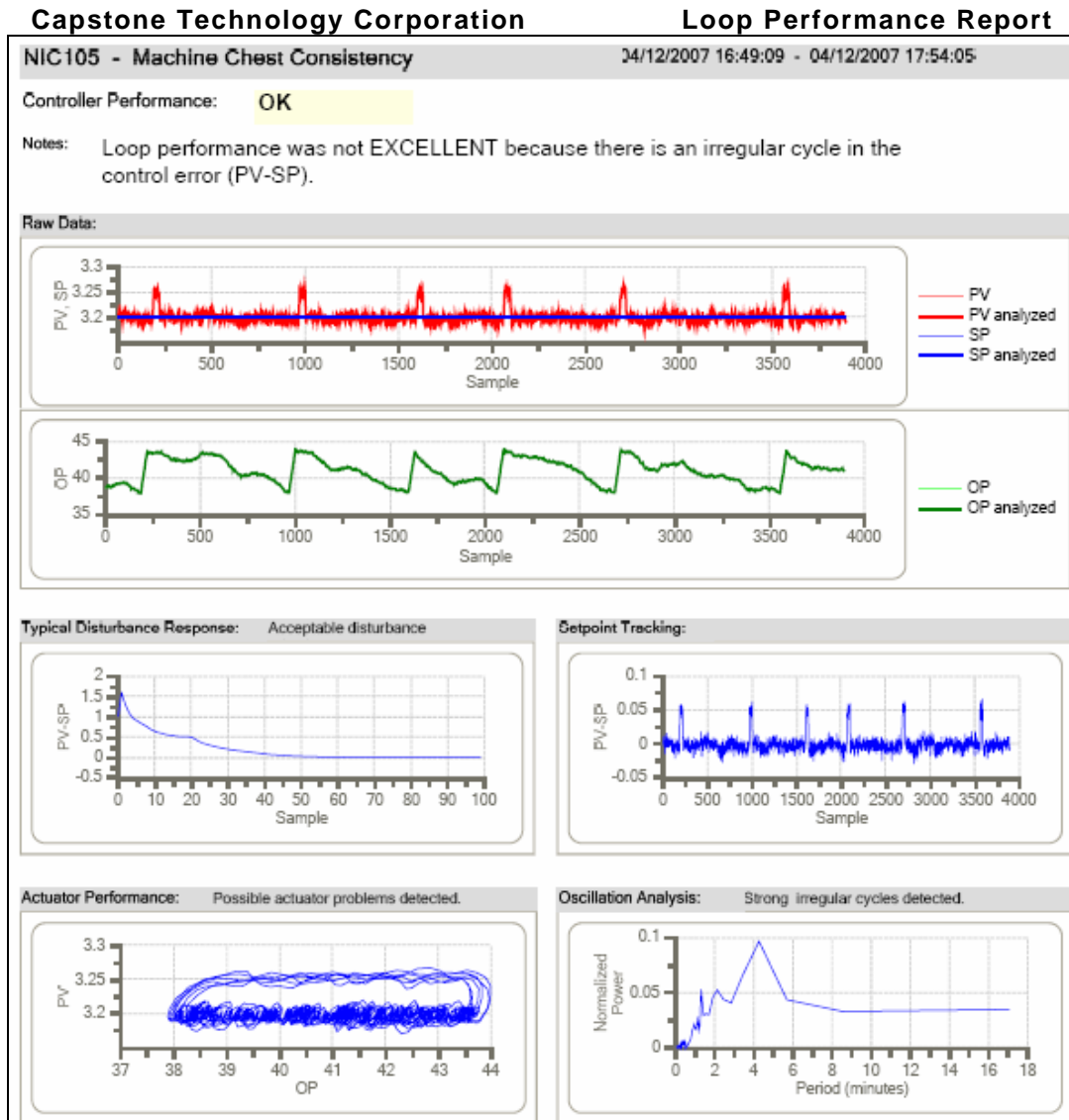
Figure 4 Loop performance report
