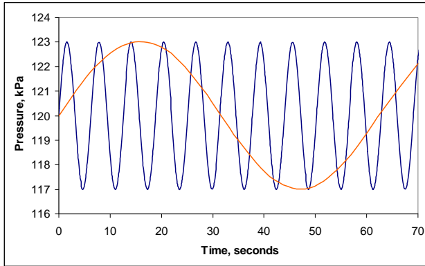
Figure 9 Aliasing due to slow sampling
