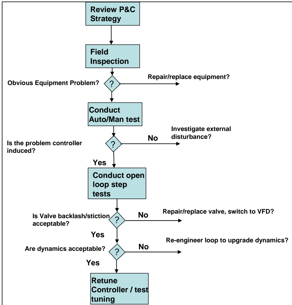
Figure 11 Control Loop Troubleshooting Flowchart
